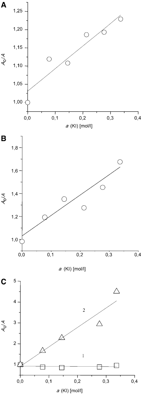
FIGURE 2 Stern-Volmer plots for KI quenching of main log-normal components belonging to tryptophan residues in fluorescence spectra of mutants W100F (A) and W77F (B) and wild-type OEP16 (C). The plots 1 and 2 in C correspond to the components plotted as spectra 2 ( \lambda_{\text{max}} = 336.2 nm) and 3 ( \lambda_{\text{max}} = 340.0 nm) of Fig. 1 D , respectively. Abscissas: chemical activities of KI. Ordinates: the ratio of full areas (integrals) under component spectra measured without KI ( A_0 ) and at a given quencher activity a (A). Points (○) are calculated A_0/A versus a ; the straight lines are the linear regressions of the points. See also Table 1 for results.
